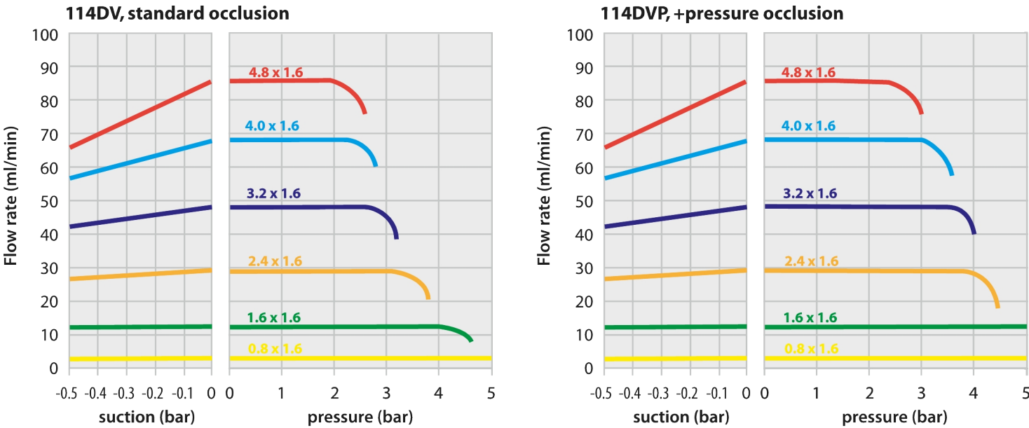
Flows obtained pumping water at 100rpm CCW-rotation
