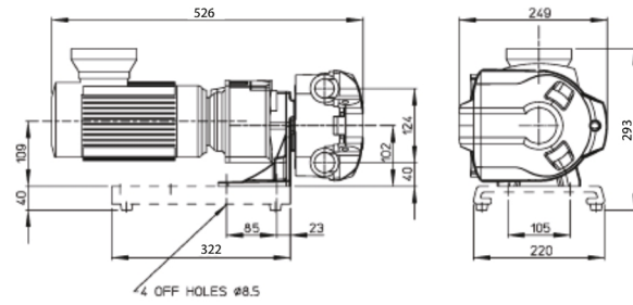
79 rpm model
