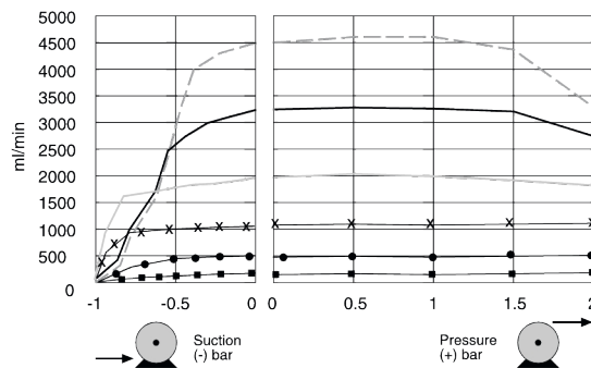
521R2C Pumphead performance curve, with Marprene tubing at 291rpm
