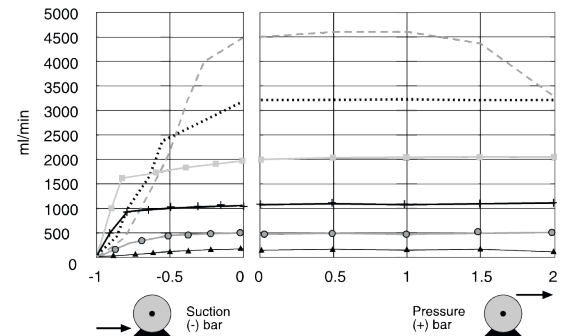
521R2C Pumphead performance curve, with Marprene tubing at 291rpm
