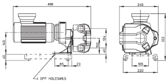
245 rpm model
