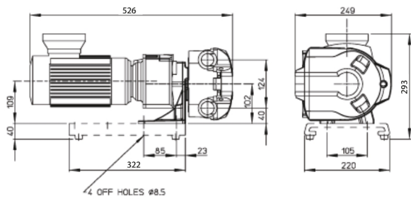
79 rpm model
