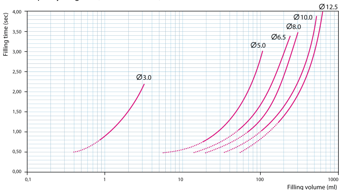
PF22 – capacity diagram (based on water)
